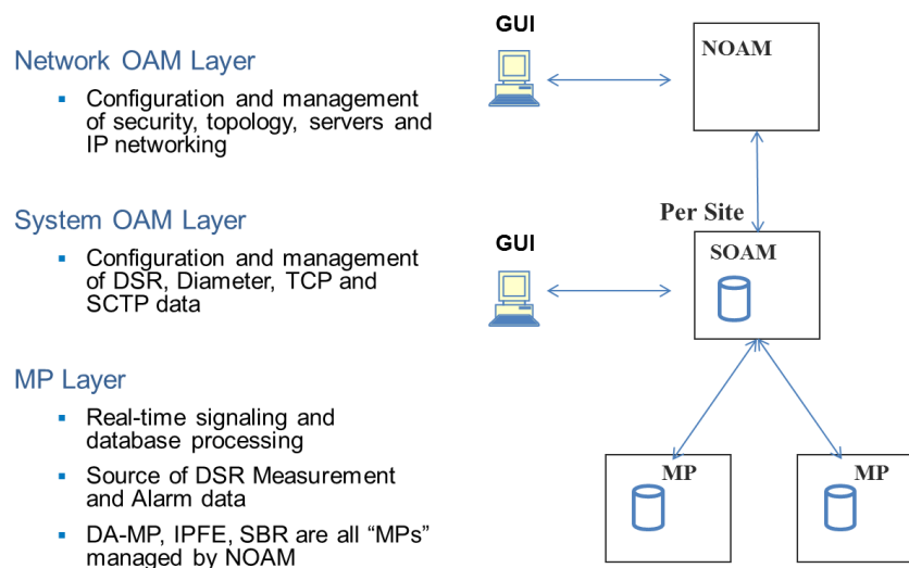
Figure 3: Three Tier OAM Topology
